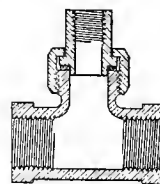
Fig. 3156. CARBURETOR UNION-TEE.
